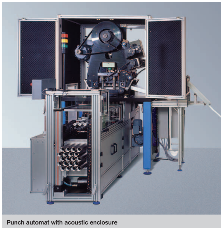
Acoustic protection cabin
