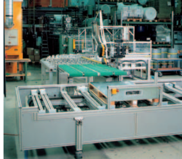
Automatic palletizing plant
