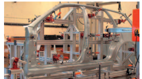
Clamping and measuring device
