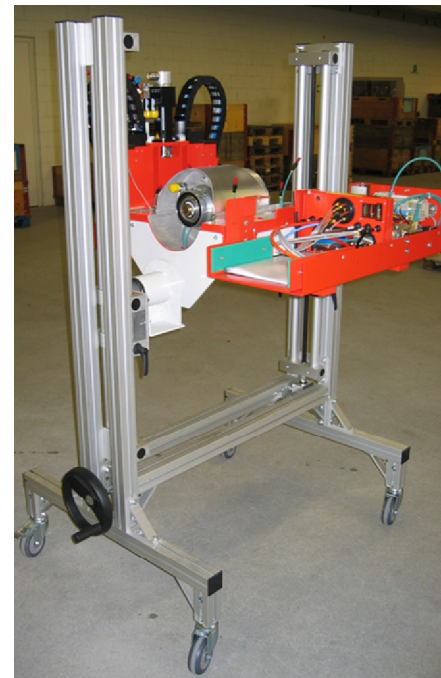
Assembling cart (adjustable for height)
